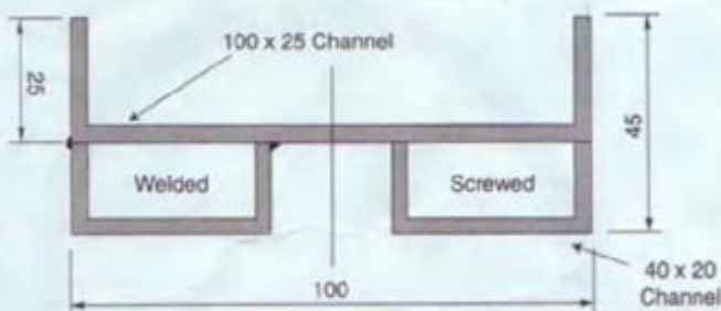
Example of channel combination to allow a removable bead
