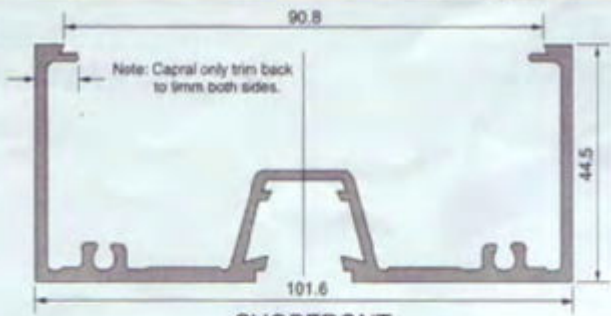
SHOPFRONT Rolled with glazing bead on inside
