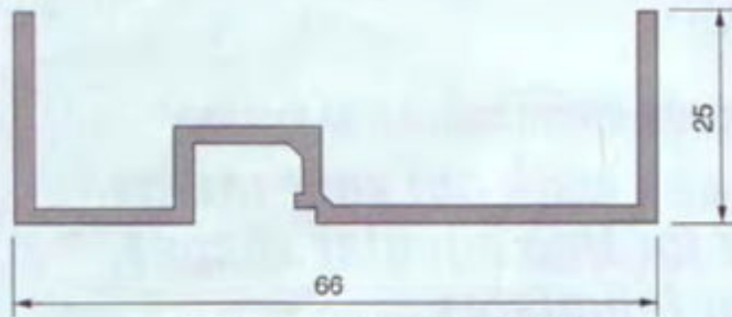
COMPACT WINDOW SECTION Rolled with glazing bead on inside
